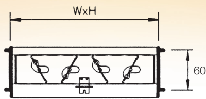
G1 Sectional View
